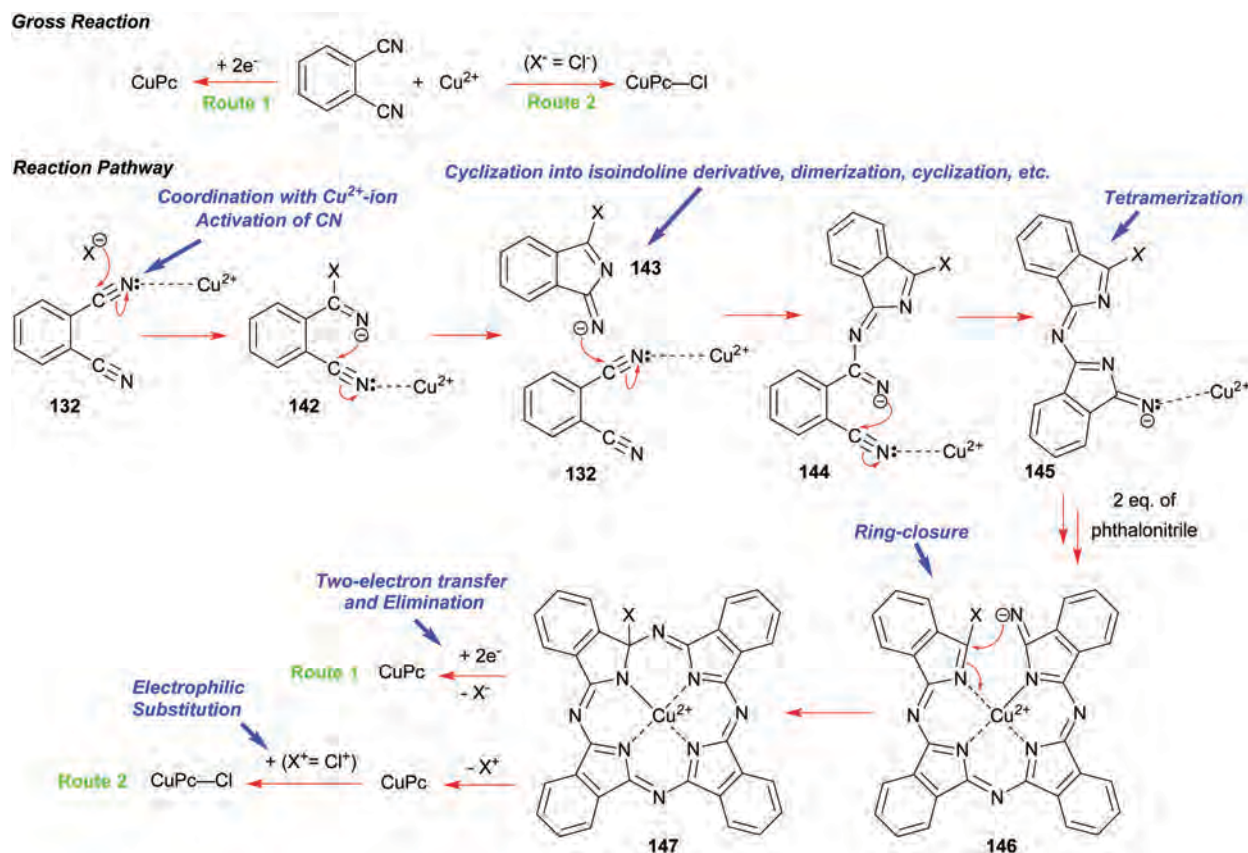
Scheme 22 Synthetic pathways to CuPc 141 and CuPc-Cl starting from phthalonitrile.
