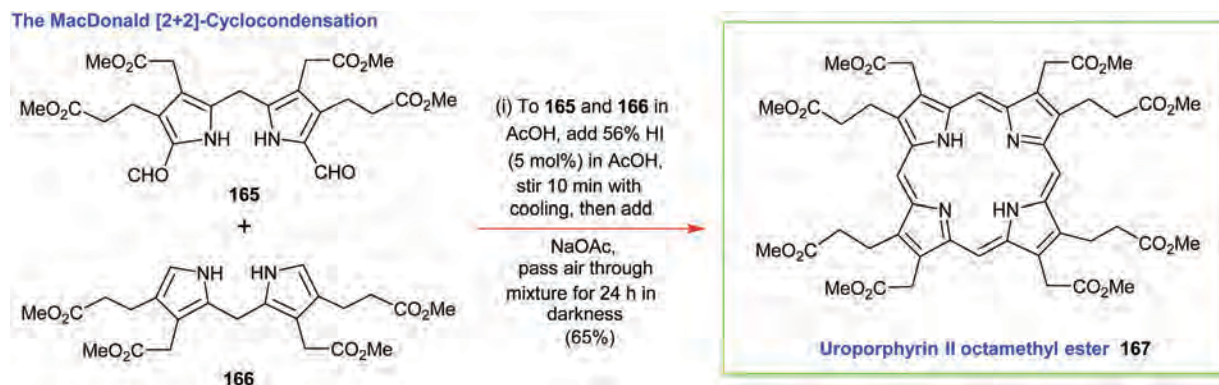
Scheme 25 MacDonald's [2+2]-cyclocondensation route to uroporphyrin II octamethyl ester 167 .
